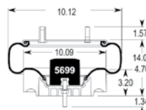
Cross Section
