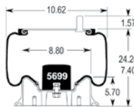
Cross Section
