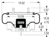
Cross Section
