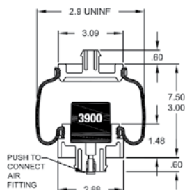
Sleeve FIRW02-358-7206
