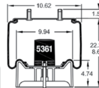
Cross Section
