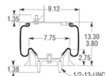
Cross Section
