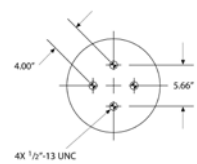
Piston Bottom View
