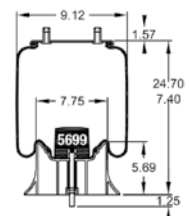
Cross Section
