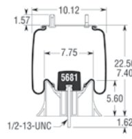
Cross Section
