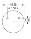
Bead Plate Top View
