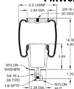
Sleeve FIRW02-358-7036
