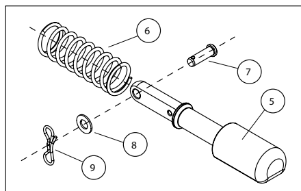
SLIDER PIN
