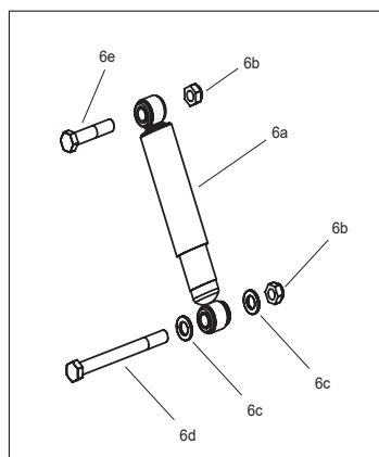
SHOCK ASSEMBLY
