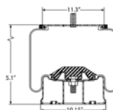
Cross Section
