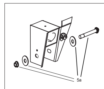
HANGER ASSEMBLY
