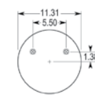
Bead Plate Top View
