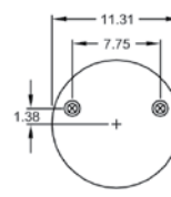
Bead Plate Top View
