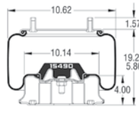
Cross Section
