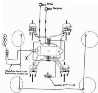
Air Control Piping: Single Height Control Valve & External Dock Lock
