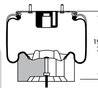
Cross Section
