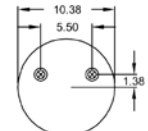
Bead Plate Top View
