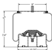
Cross Section
