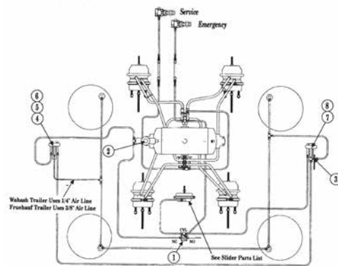
Air Control Piping: Dual Height Control Valves & External Dock Latch
