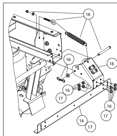
MUD FLAP MOUNTING
