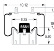
Cross Section
