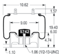
Cross Section
